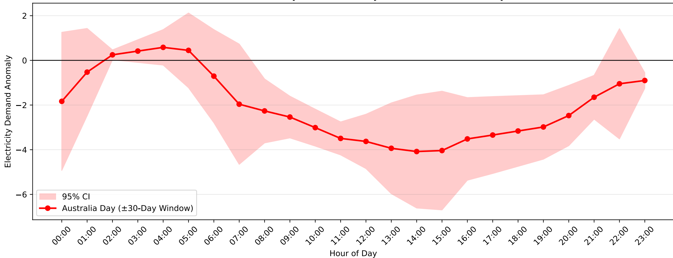
Bass Hill Demand Anomaly: Australia Day (2005-2006, \pm 30 -Day Window)
