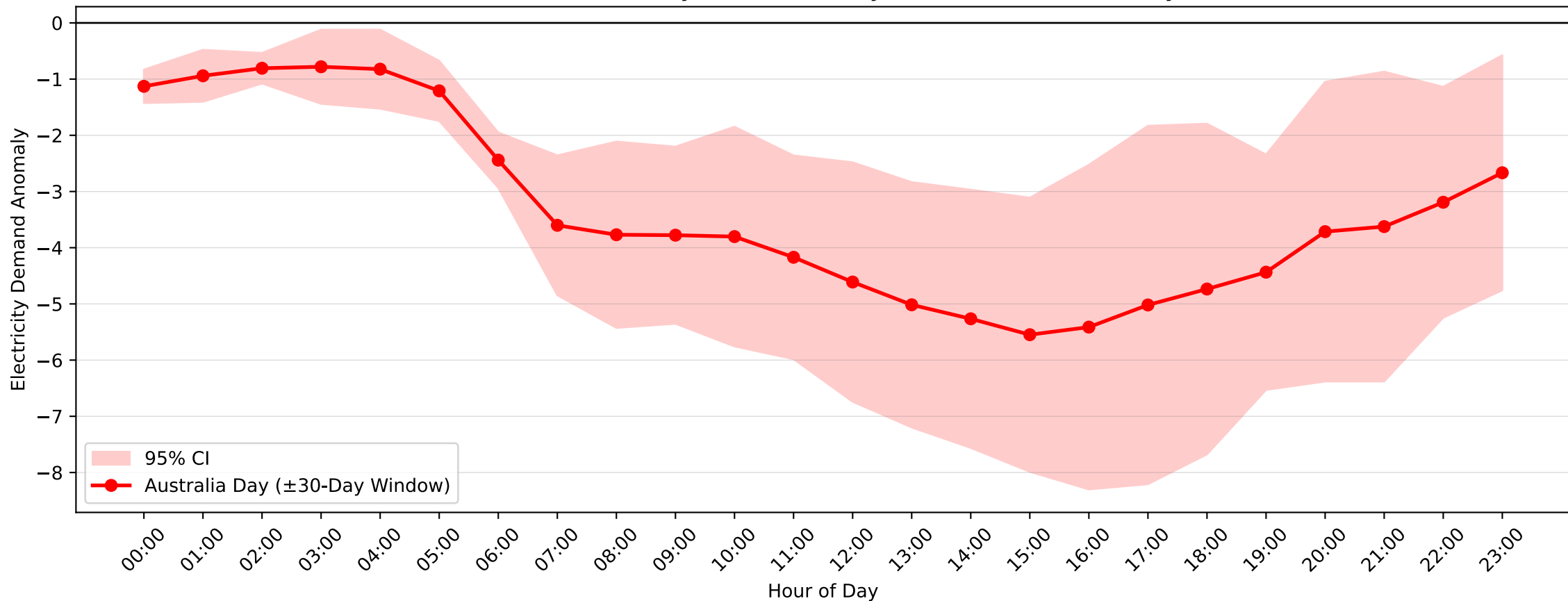
Bass Hill Demand Anomaly: Australia Day (2016-2017, \pm 30 -Day Window)
