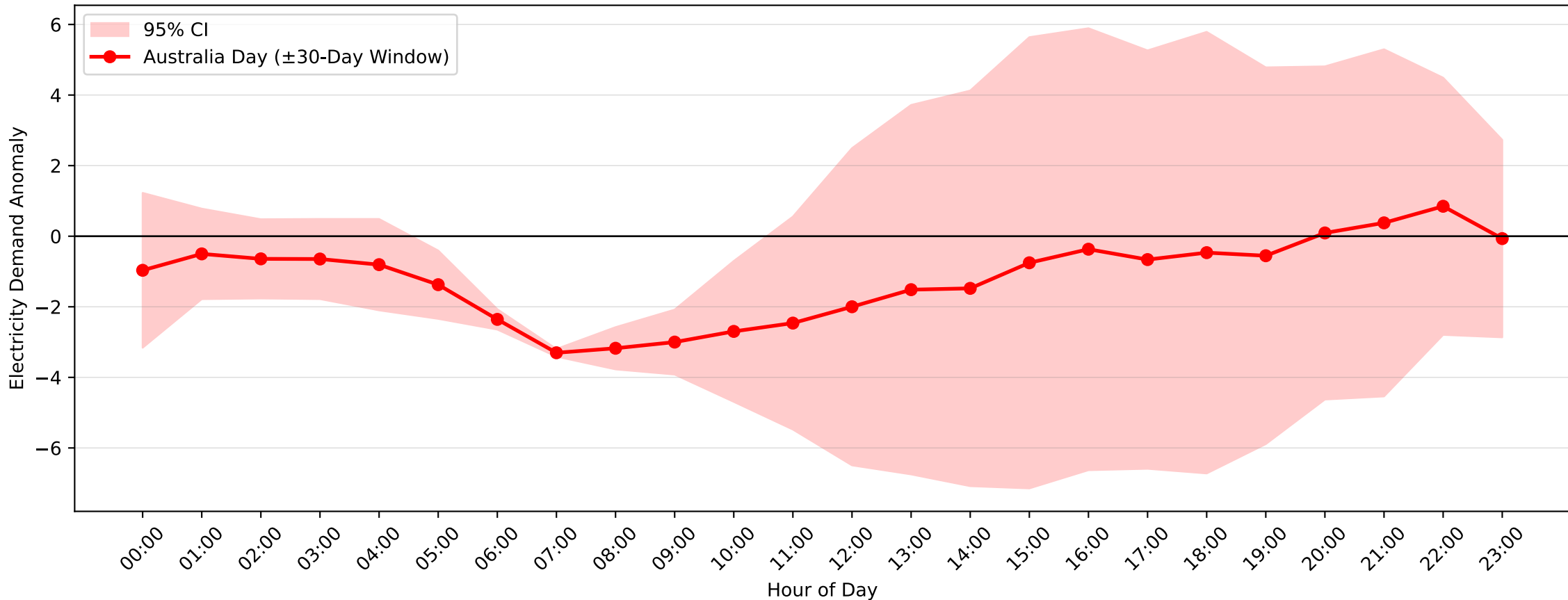
Bass Hill Demand Anomaly: Australia Day (2009-2010, \pm 30 -Day Window)
